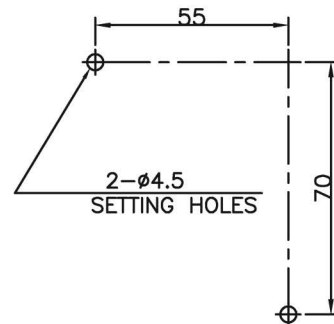
SETTING DIMENSION
